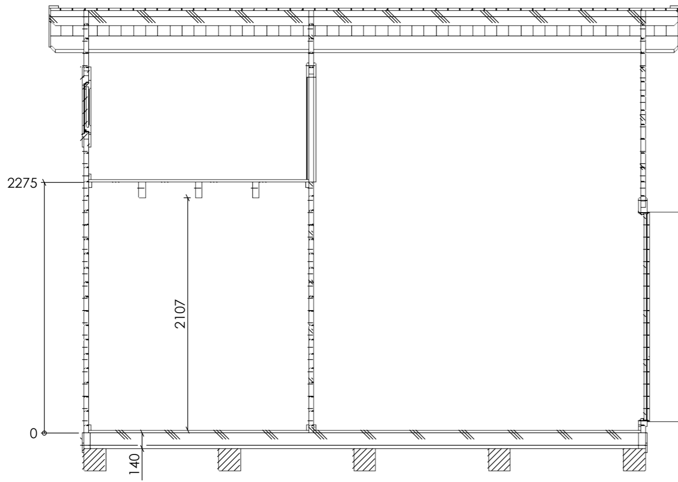
Section A
