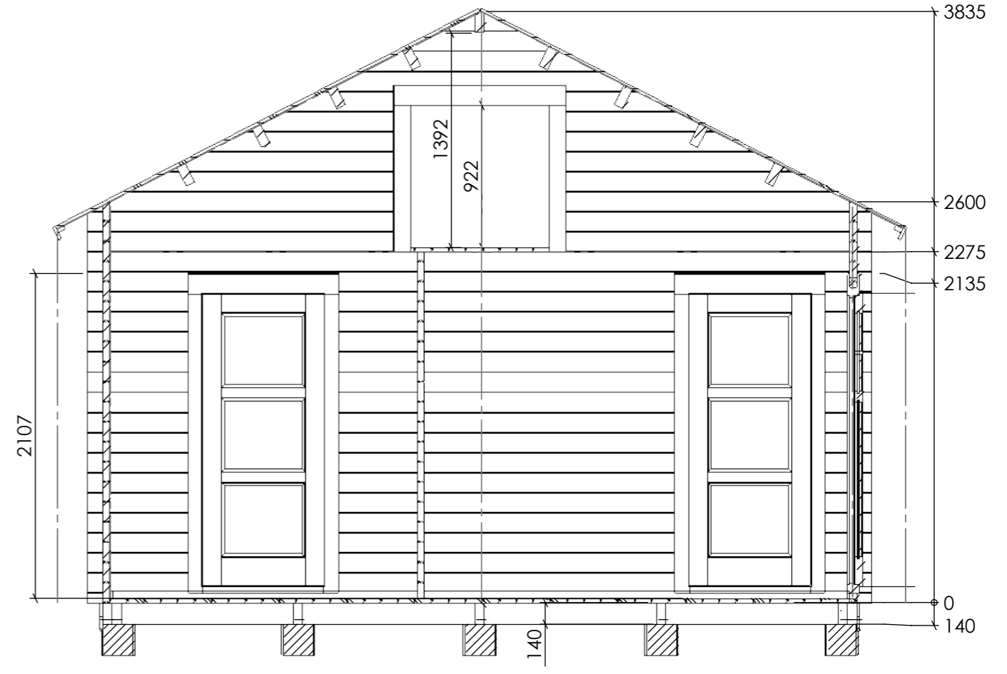
Section B
