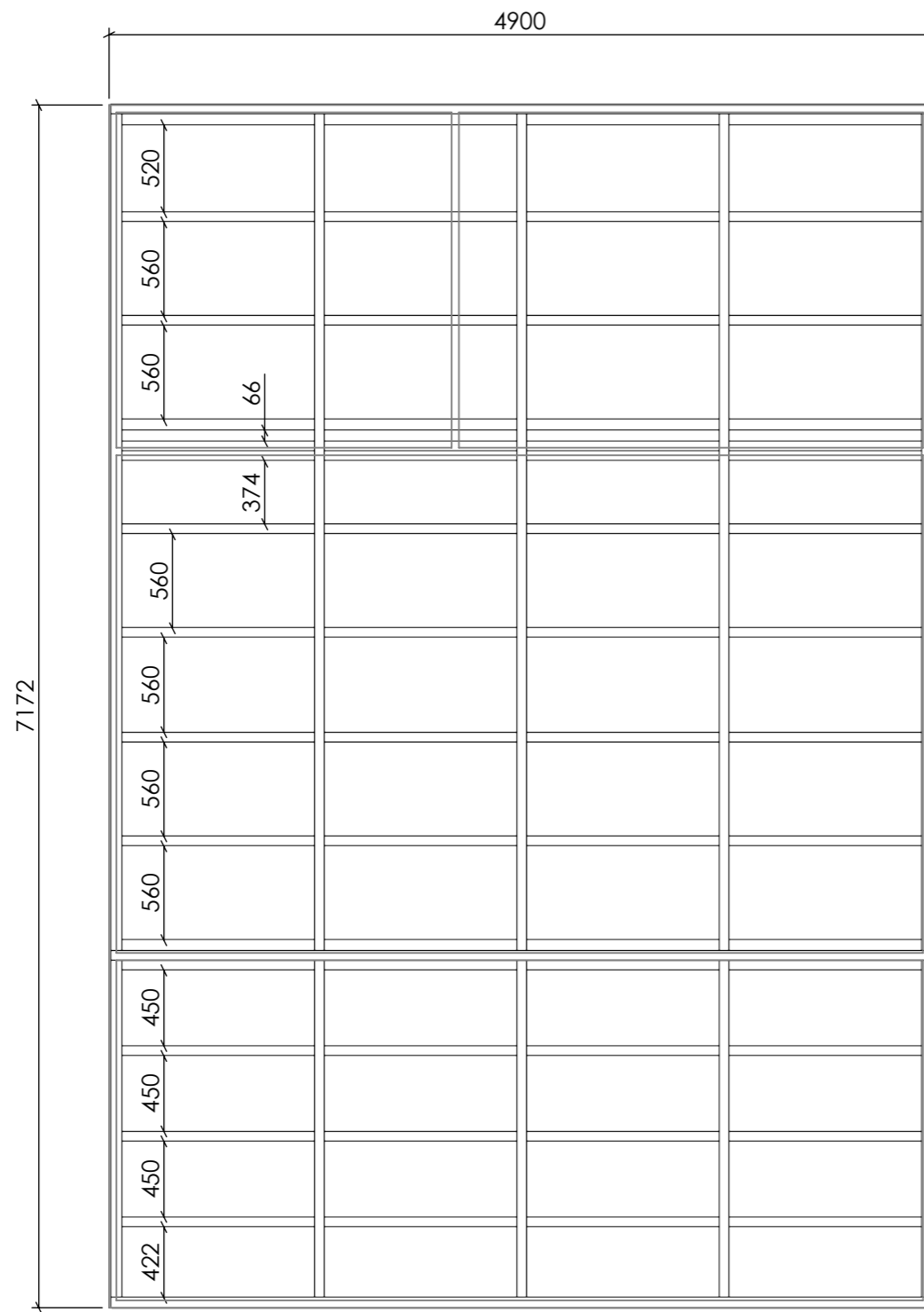
FLOOR BEAM 60X140
