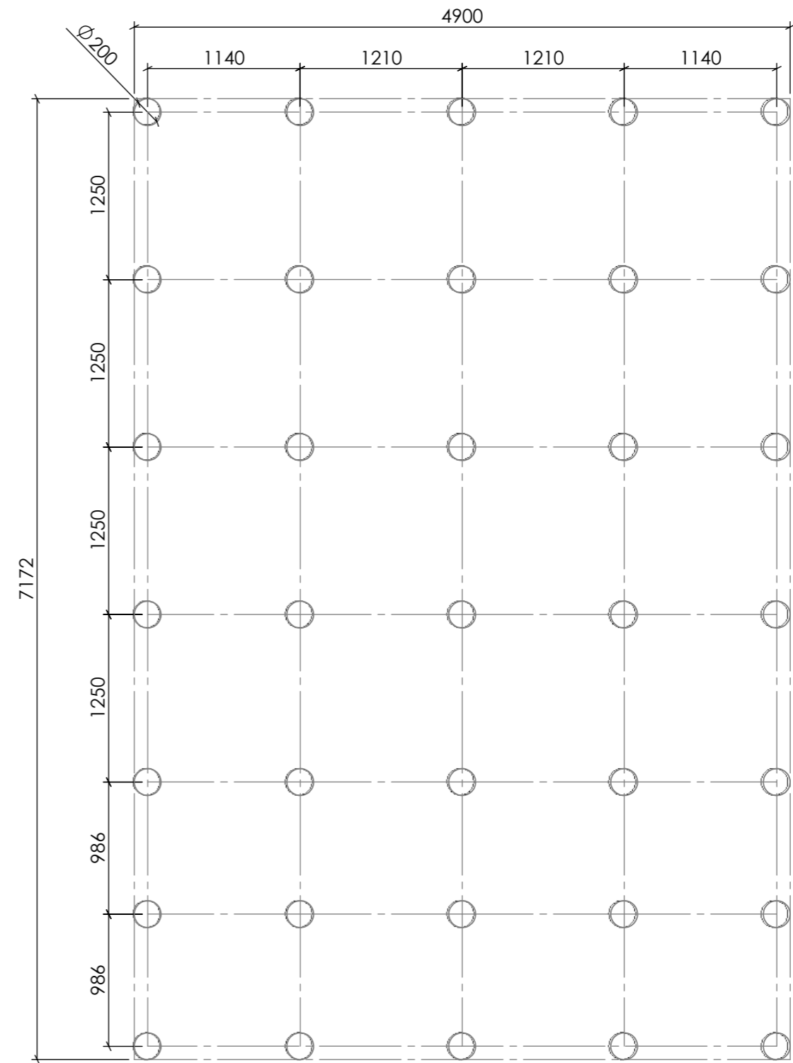
POLE PLAN
