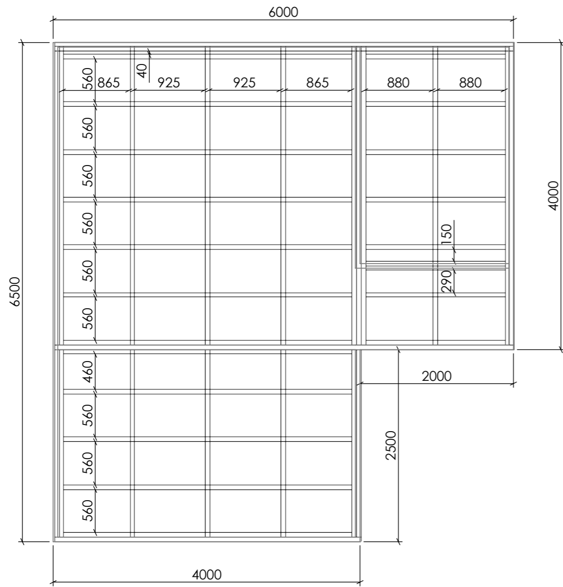
Floor Beam 60x140
