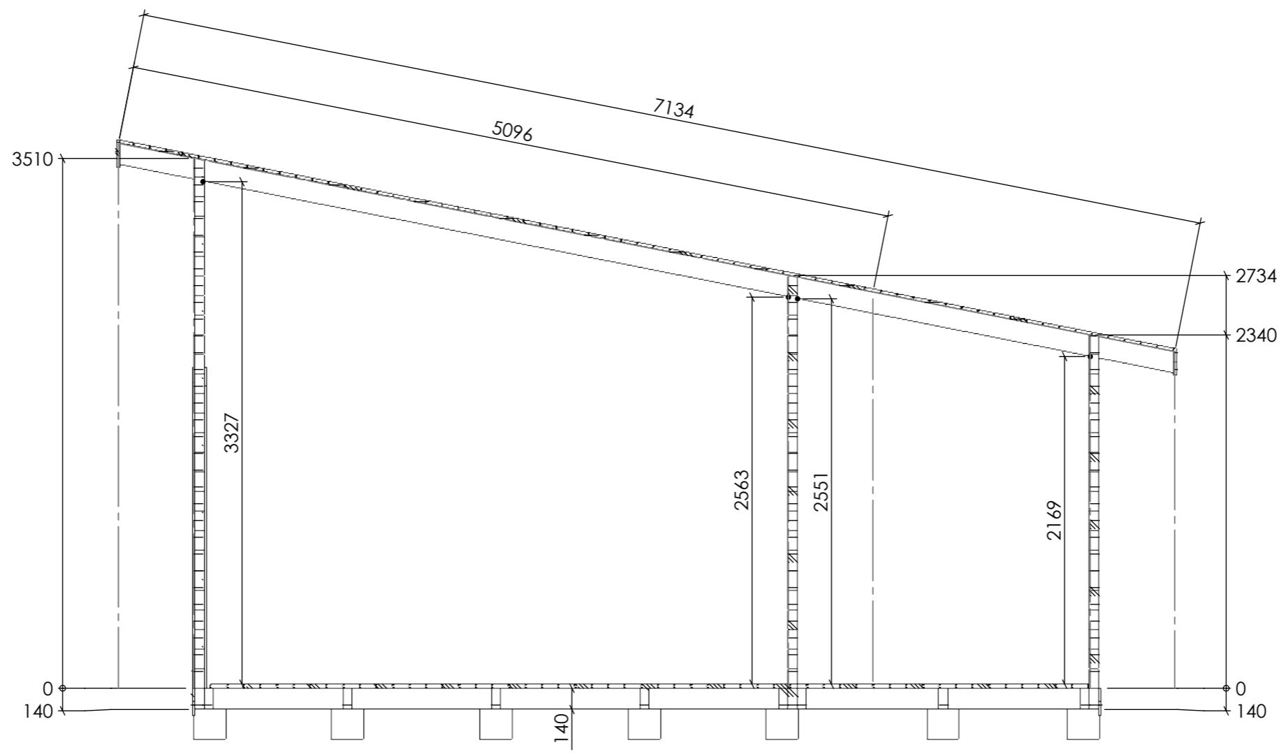
Section
