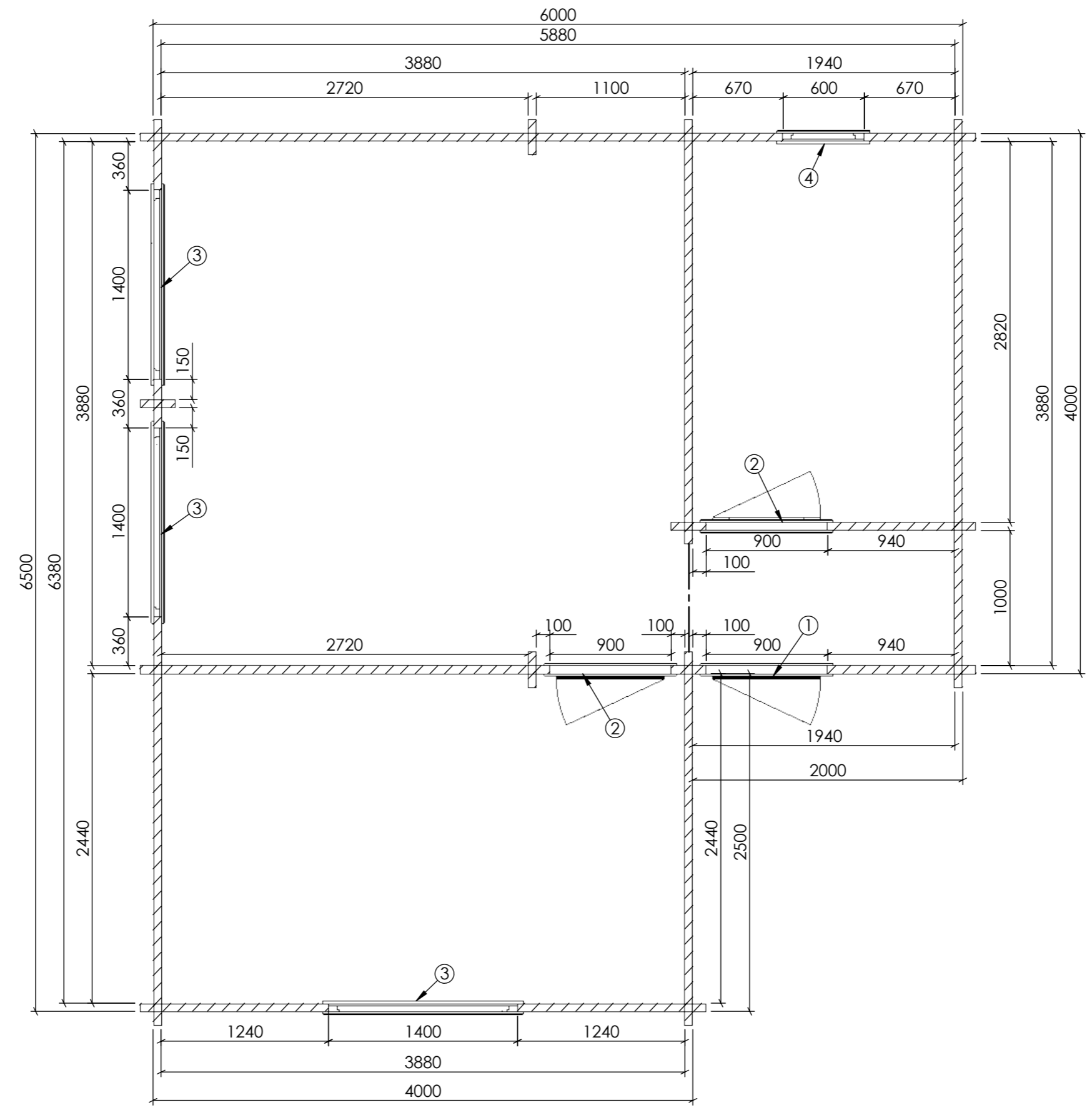
Plan
