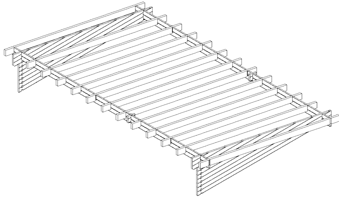
Rafters 60x180
