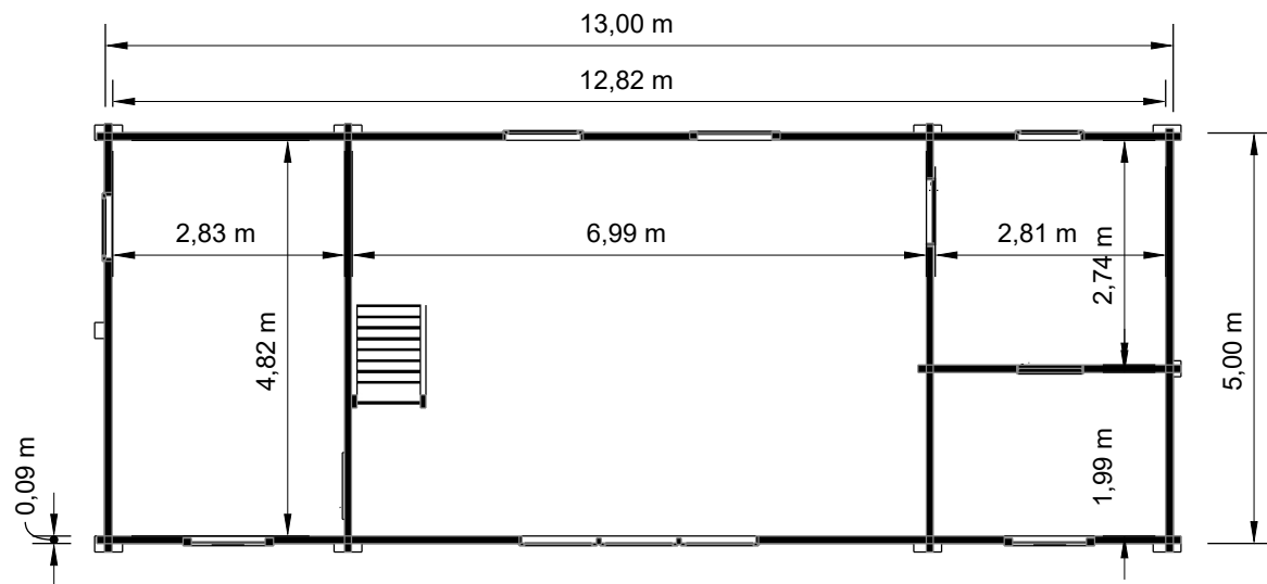
Plan 1
